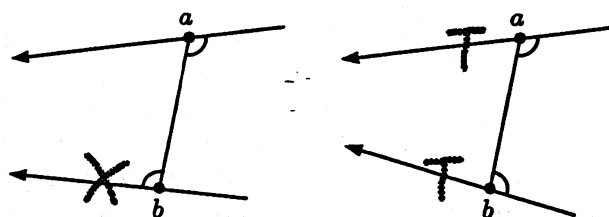
Figure 6: Cases in normal mode
