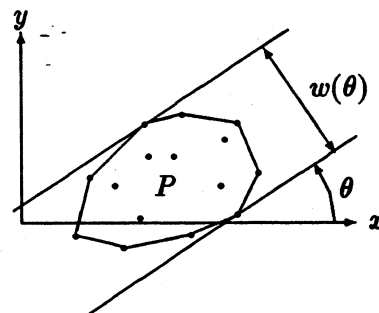
Figure 1: The function w(\theta)
