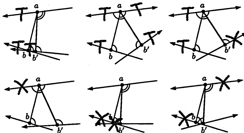
Figure 7: Cases in tentative mode
