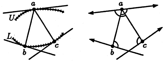
Figure 4: A fence triangle
