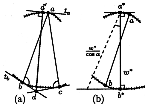
Figure 5: Under- and overestimates
