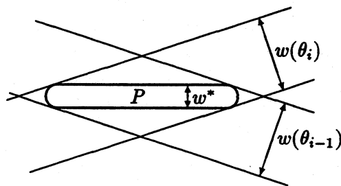
Figure 2: A bad case
