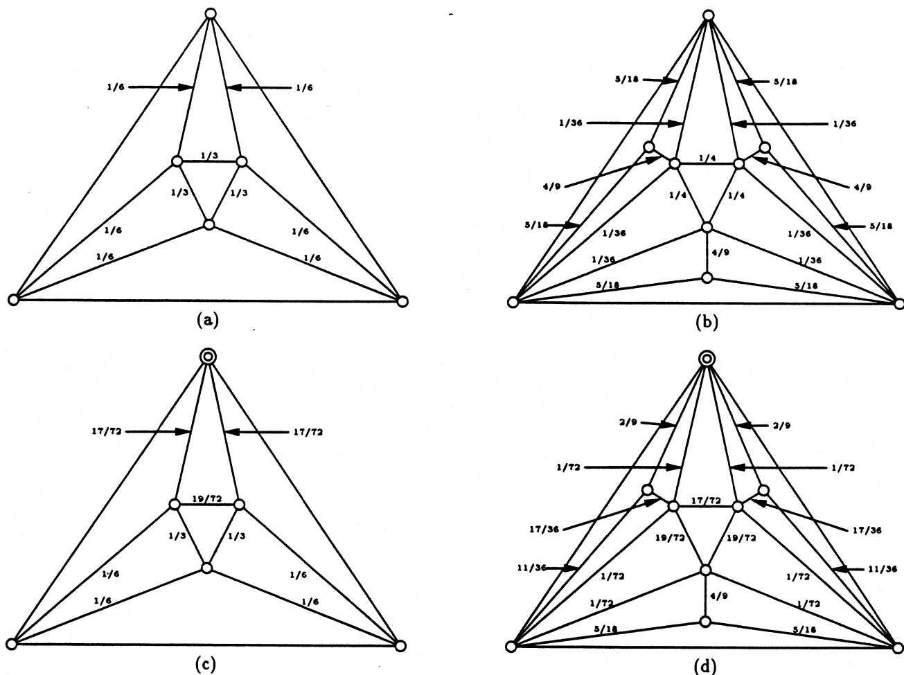
Figure 2: Construction and weight assignments used to reduce H2BPX to the Hamiltonian cycle problem for inscribable graphs. (a) A blue triangle that is not an s -triangle. (b) A red triangle that is not an s -triangle. (c) A blue s -triangle. (d) A red s -triangle. In (c) and (d), the double circle represents the s -vertex.
