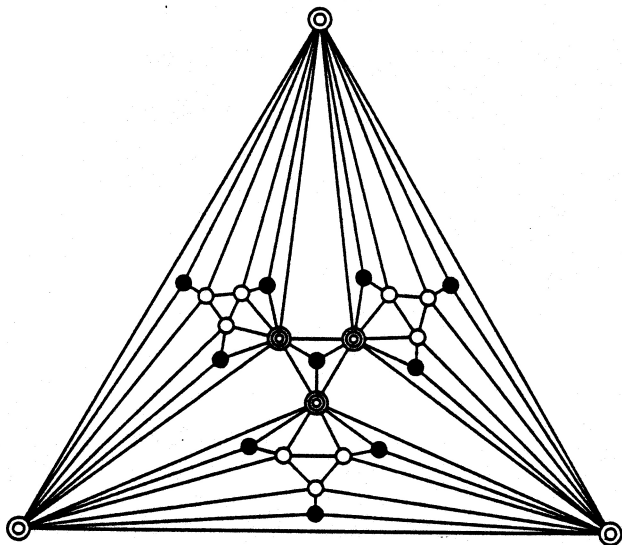
Figure 3: An inscribable graph with no 2-factor.
