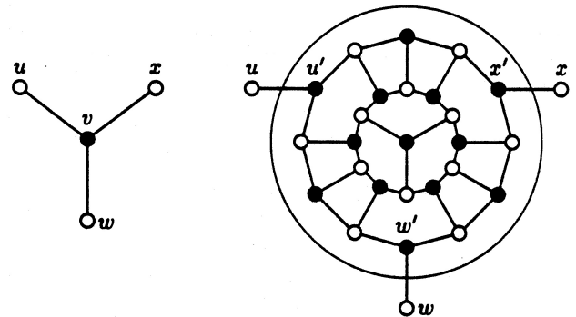
Figure 1: Construction used to prove H2BTPX is NP-complete.
