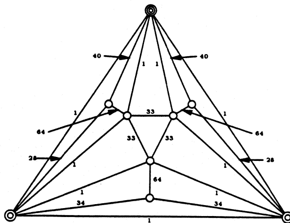
Figure 4: Edge weightings for the graph of Figure 3.
