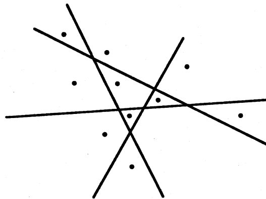
A set of ten points separated by four lines Figure 1
