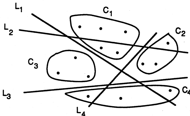
A possible cluster set for a set of fourteen points P and four lines H = \{L_1, L_2, L_3, L_4\} . C_1 is a cluster of (P,H) determined by \{L_1, L_4\} . Figure 2.
