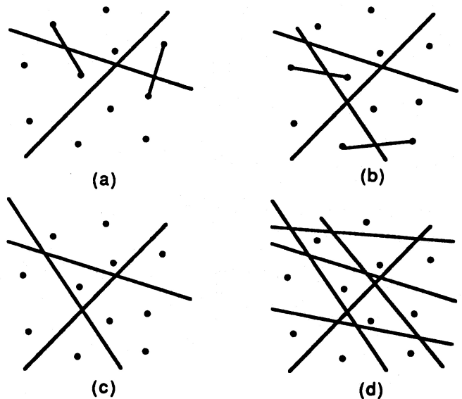
The sequence of the first three 2-splits ((a), (b), and (c)) of P and the final separating set of lines of P (d).
