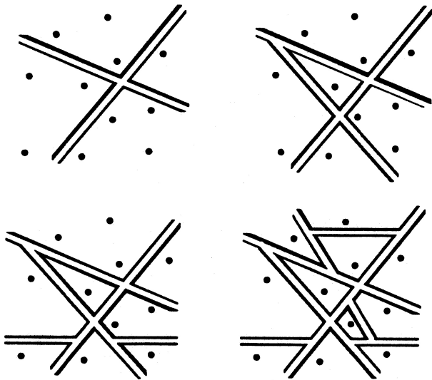
The polygons corresponding to each cluster after the addition of separating lines. The points and lines are as in Figure 3. Figure 4
