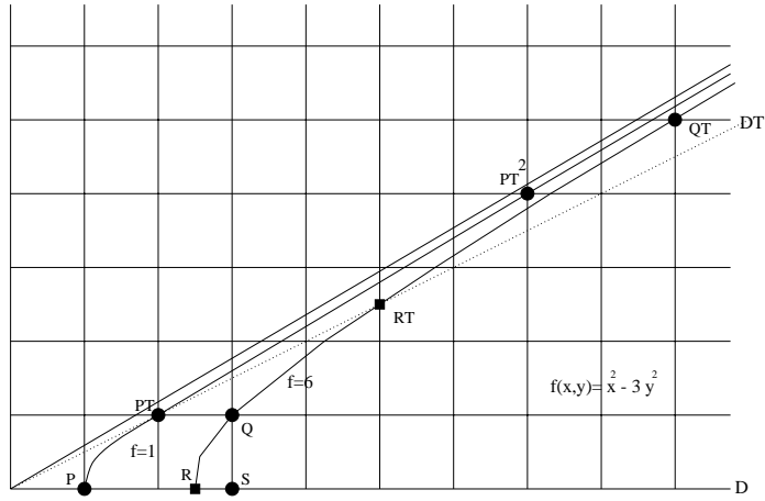
Figure 1: Hyperbolæ f(x,y) = x^2 - 3y^2 = \delta . Cases \delta = 1 and \delta = 6 . For \delta = 1 , \{P\} is the initial pattern, PT, PT^2 \dots \in i.c.h. For \delta = 6 , \{S, Q\} is the initial pattern.
