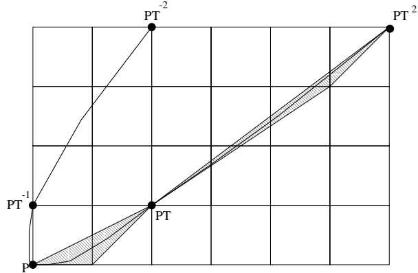
Figure 2: Parabola x^2 + y^2 - 2xy - y = 0 , \{P\} is the initial pattern, PT^{-1}, PT^{-2}, \dots, P, PT, PT^2, \dots \in i.c.h. Shaded triangles show T in action.
